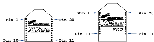
Figure 1-03. XBee/XBee-PRO RF Module Pin Numbers
